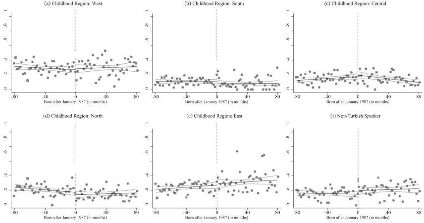
Figure 1 Balanced covariates
